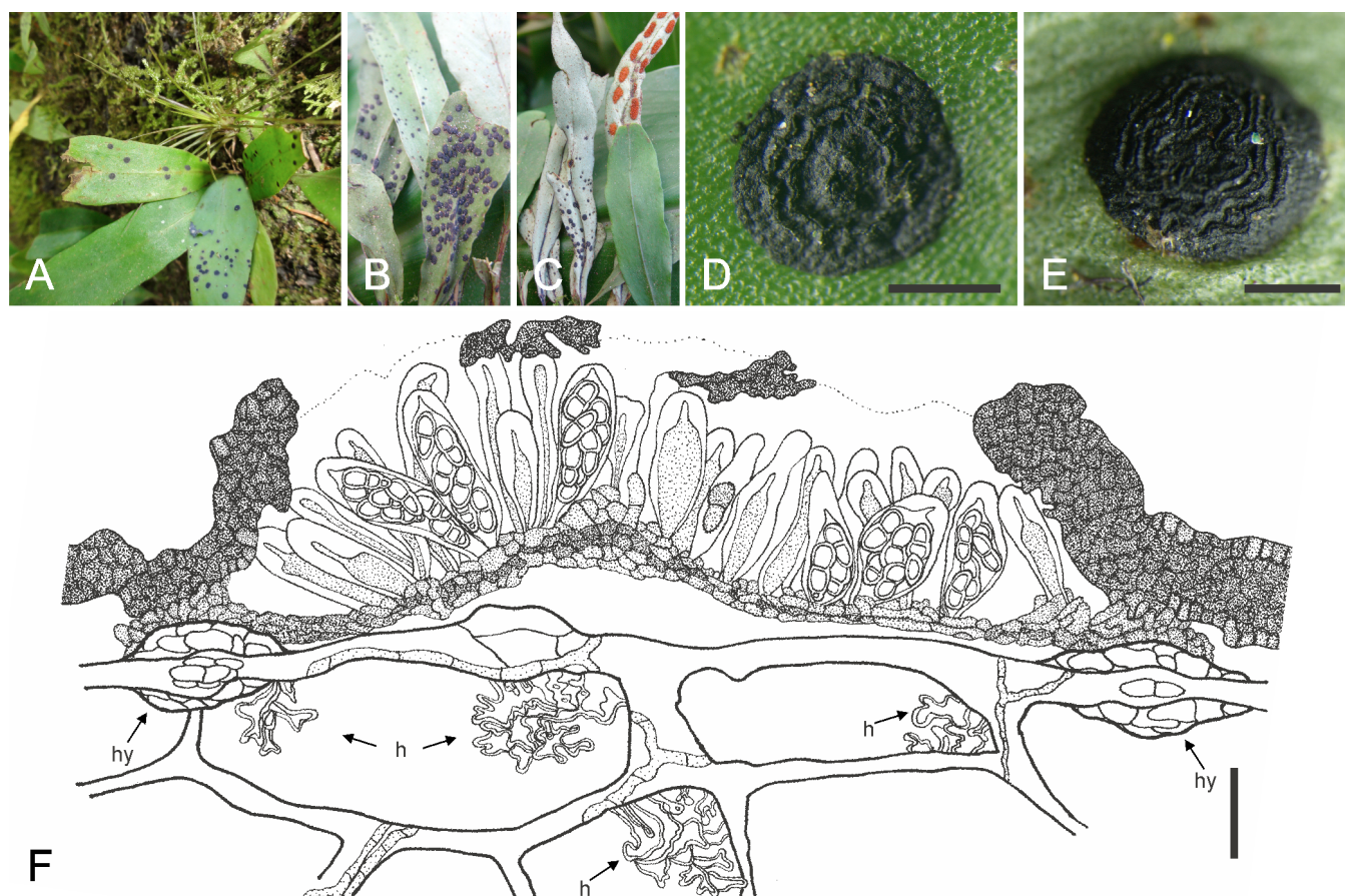
Fig. 1. Inocyclus angularis (VIC 39747). A–E. Colonies on P. astrolepis . F. Ascoma with asci and ascospores. h = coraloid haustoria, hy = hypostroma that connects the ascoma with the host tissue. Bars: D–E = 4 mm, F = 20 \mu m.
